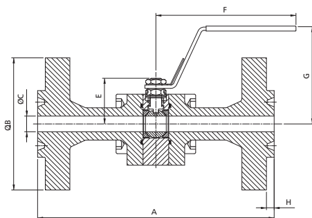
Lever operated (DN 15 - DN 25)
