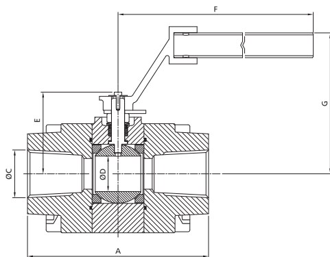
Screwed
