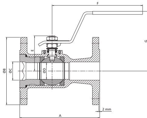
Lever operated (DN 15 - DN 65)
