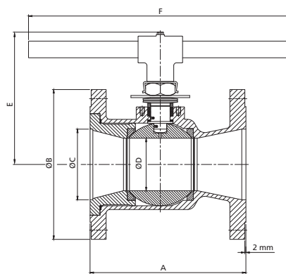
Wrench operated (DN 80 - DN 150)
