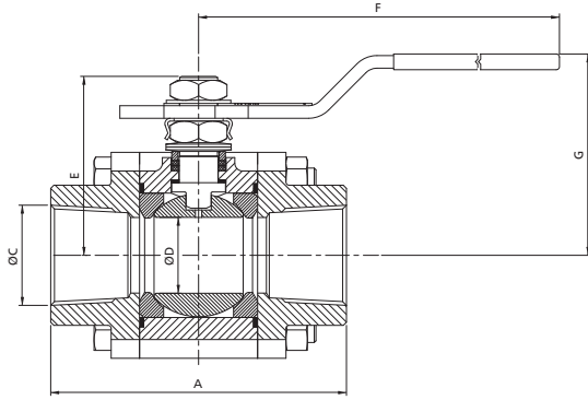
Screwed
