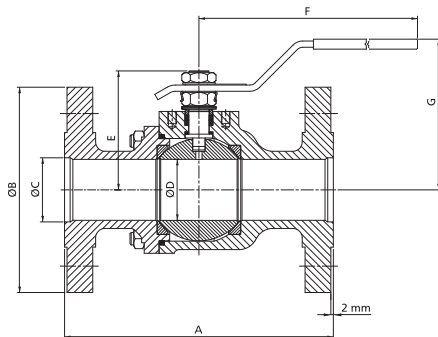
Lever operated (DN 15 - DN 50)
