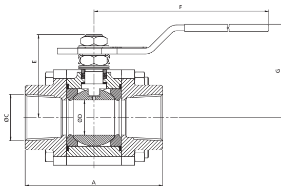
Screwed
