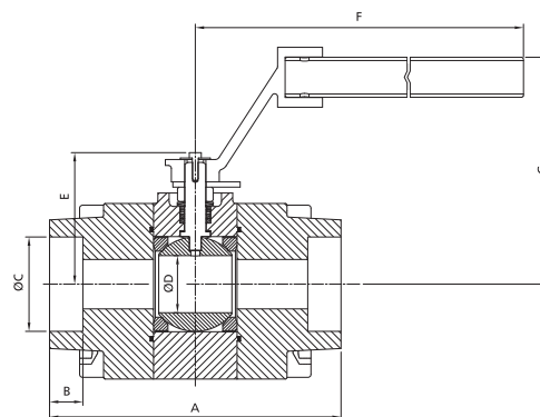
Socket-weld end
