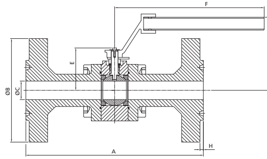
Wrench operated (DN 40)
