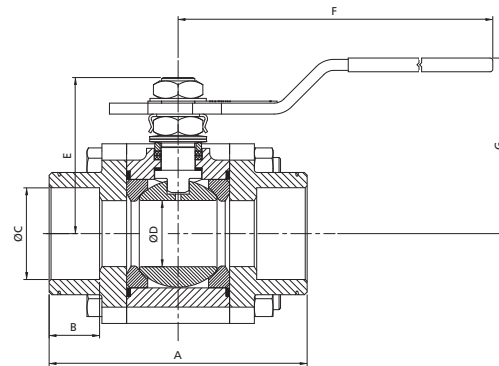
Socket-weld end
