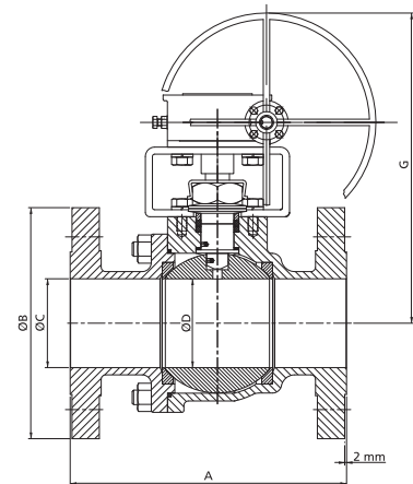
Gear operated (DN 100 - DN 200)
