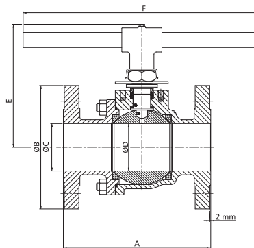
Wrench operated (DN 65 - DN 200)
